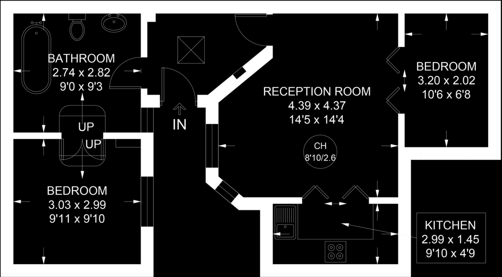
LOWER GROUND FLOOR
